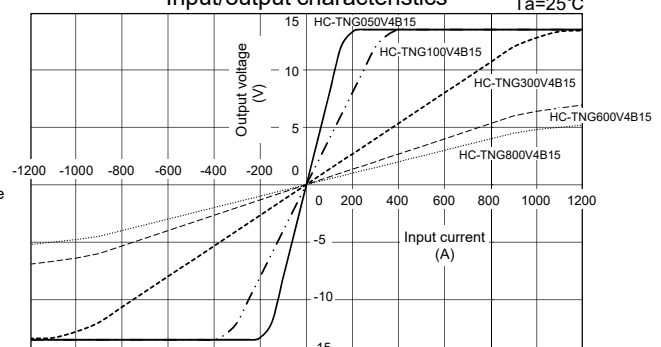
Input/output characteristics
