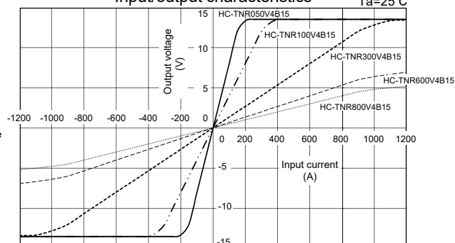
Input/output characteristics
