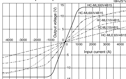
Input/output characteristics
