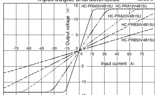
Input/output characteristics
